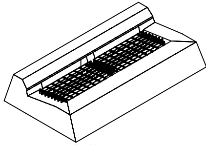
TYPE "C" BIT CURB
