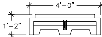
END VIEW (CENTER SECTION) (WALL THICKNESS IS 3'') (ROOF THICKNESS IS 5 1/2'', 7 1/2'' @ BEAMS)
