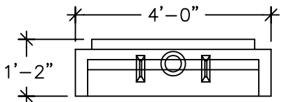
END VIEW (END SECTION) (WALL THICKNESS IS 3'') (ROOF THICKNESS IS 5 1/2'', 7 1/2'' @ BEAMS)
