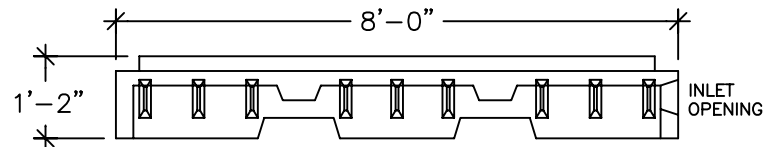
SIDE VIEW (WALL THICKNESS IS 3'') (ROOF THICKNESS IS 5 1/2'', 7 1/2'' @ BEAMS)
