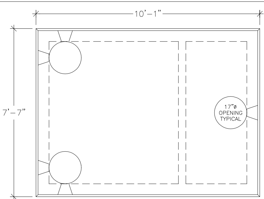
TOP VIEW (COVERS REMOVED)
