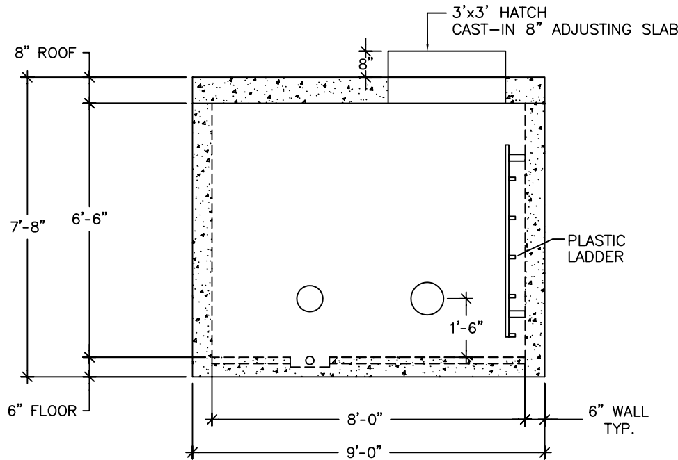
SIDE VIEW
